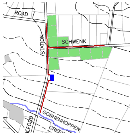
Figure 4 - Package Plant for Schwenk Road
