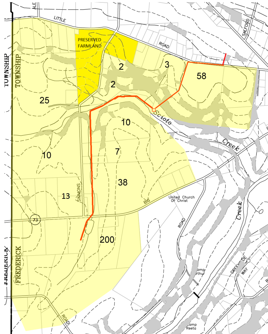
Figure 7 - Pump Station Along the Scioto Creek
