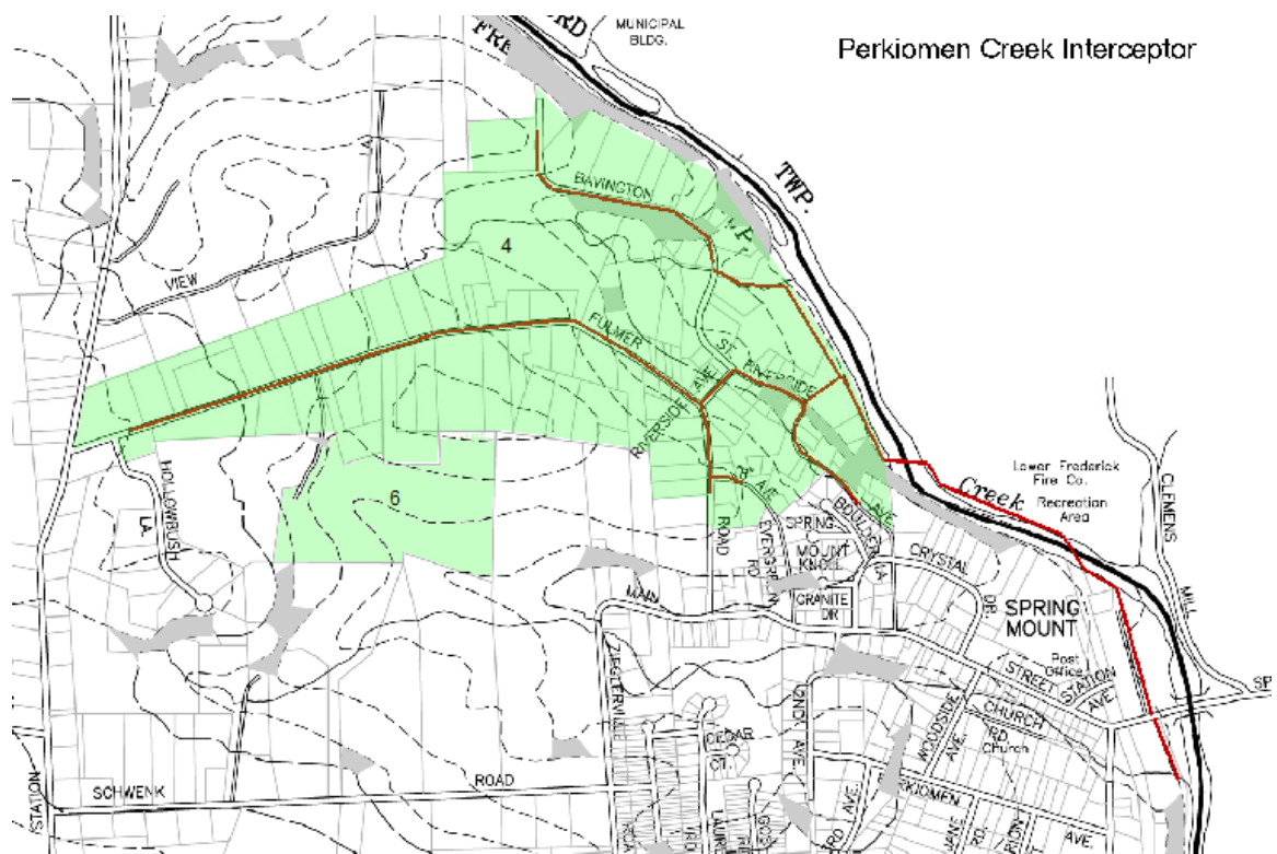
Figure 10 - Perkiomen Creek Interceptor
