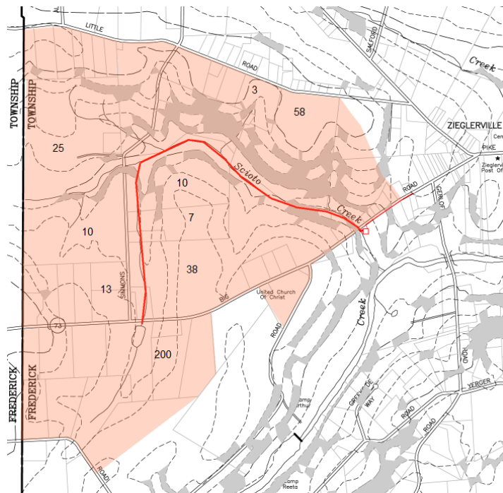
Figure 6 - Pump Station along Big Road
